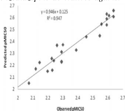
Figure 1. Plots of Predicted V/S Experimentally observed inhibitory activity of 2,4-disubstituted-1,5-benzodiazepine derivatives against E.coli .
