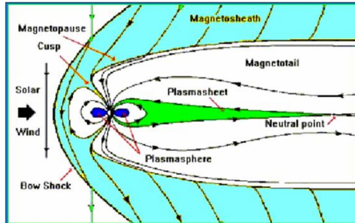
Figure 3: Shows the formation of the magnetosphere and its different regions such as bow shock, magnetopause, magnetosheath, magnetotail, cusp, plasma sheet, plasmasphere and neutral point.
