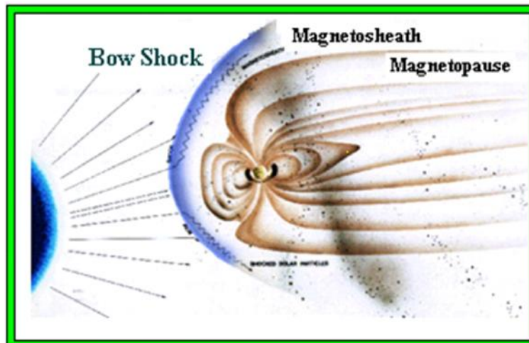
Figure 4 : Shows the formation of the bow shock front. In this figure bow shocks are formed on frontal surface of the magnetosphere, where the solar wind has its first impact with geomagnetic field.
