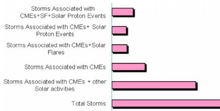
Figure 2: Shows the association of 158 large geomagnetic storms with coronal mass ejections.
